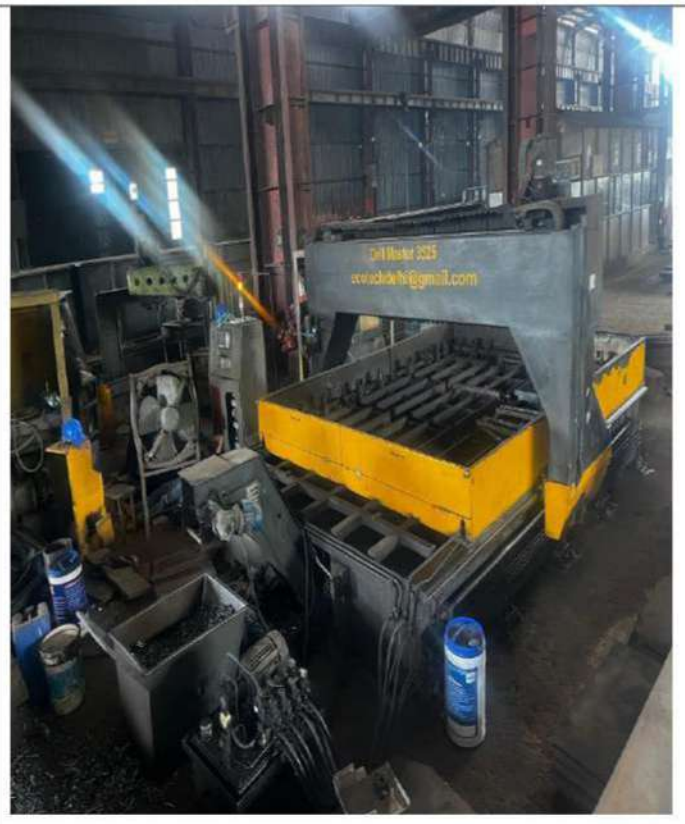
CNC DRILLING
