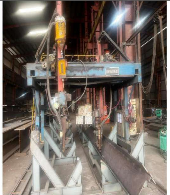
BOX WELDING SAW MACHINE
